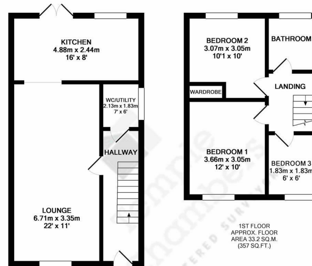
GROUND FLOOR APPROX. FLOOR AREA 45.3 SQ.M. (488 SQ.FT.)
